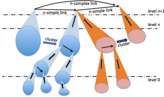
Fig. 4. Two ramifications of M , with simple and complex links
